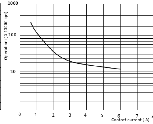
ENDURANCE CURVE
