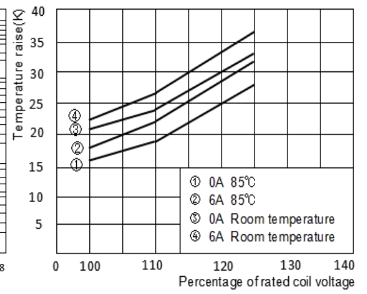
Coil temperature rise
