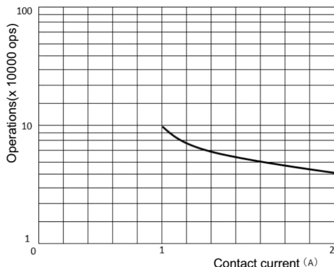
ENDURANCE CURVE
