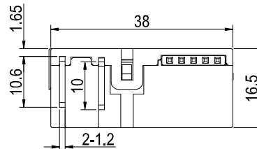
B Type Double Coils
