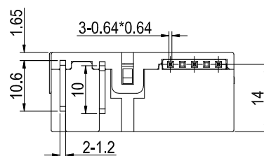
A Type Double Coils
