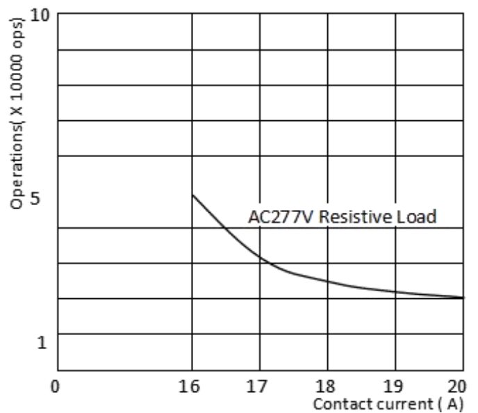
ENDURANCE CURVE
